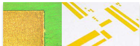
Solder mask removal (L) and coverlay kiss-cuts (R).
