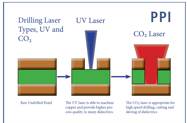
Figure 1: Drilling Laser Types
