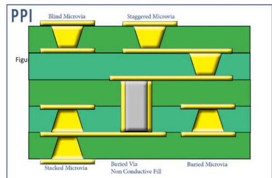
Figure 2: Via Types
